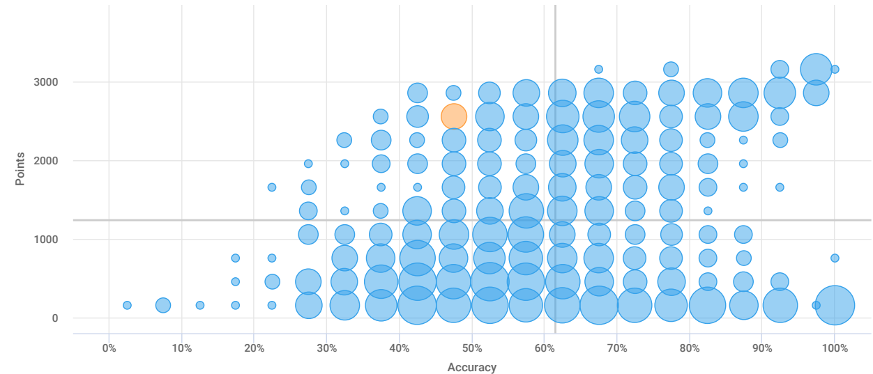
Composite Performance
